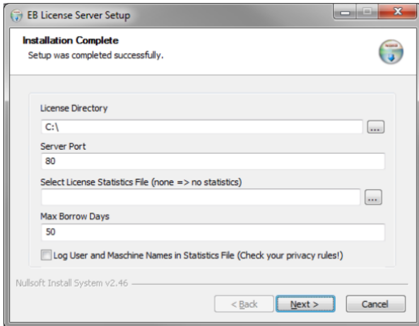
Figure 2.1: Installation dialog
